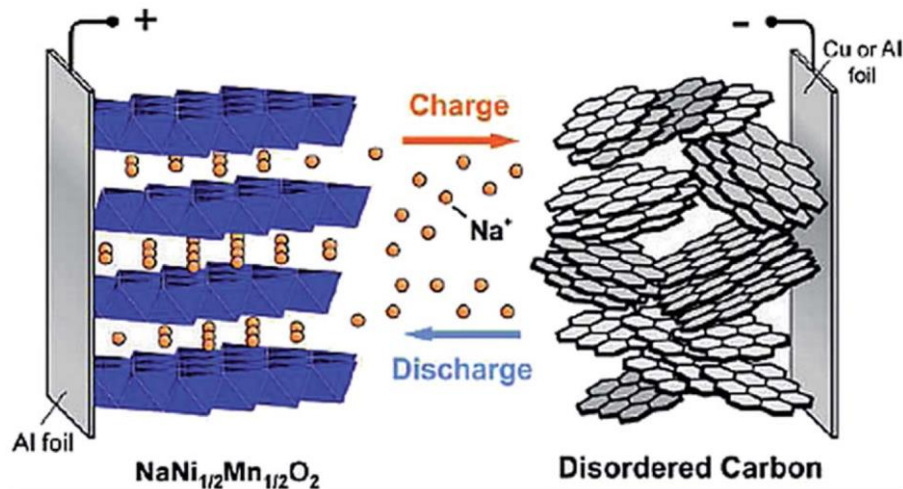
FigureA.4 - Schematic of sodium ion batteries with a layered transition metal oxide cathode and carbonaceous anode [28]
