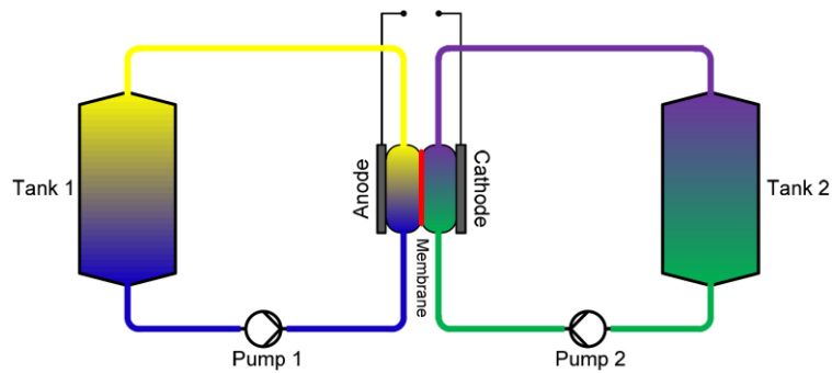
FigureA.3 – Schematic design of a redox-flow battery [25]
