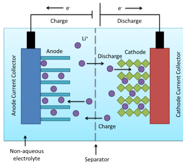
Figure A.2 - Schematic intercalation and de-intercalation of lithium in anode / cathode of a lithium-ion battery cell [22]
