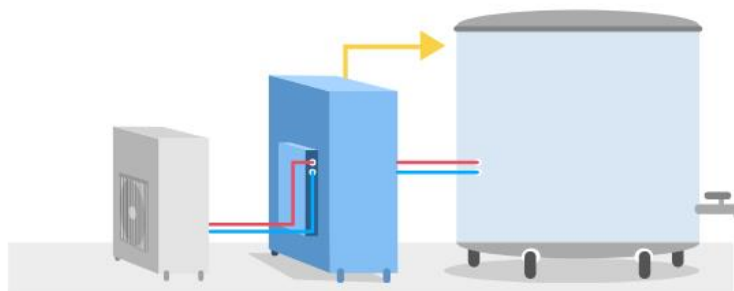
Figure A.6 – Sample cold storage technology, where cold store (middle) was cooled via compressor (left) when electricity was available (in parallel to cooling the tank) and directly cools tank (right) during an outage without requiring electricity.
