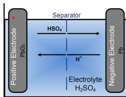
Figure A.1 - Principle of the discharge and charge process in a Lead-acid cell [25]
