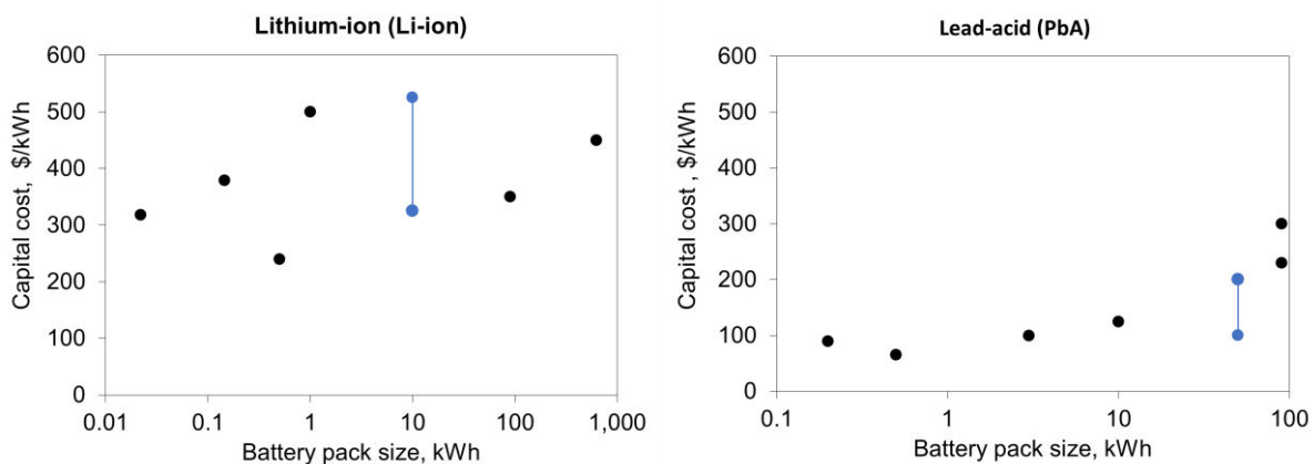
Figure 4 – Capital costs (in $ per unit capacity i.e. $/kWh) for DC-module of Li-ion (left) and PbA (right) batteries against typical battery capacity (on a logarithmic scale) as reported by interviewees (black) and according to industry standard (blue) [3,4].
