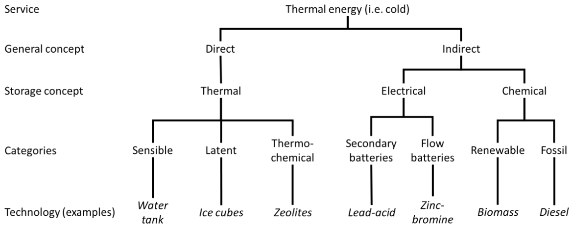
Figure A.5 – Different technology pathways to providing thermal energy.
